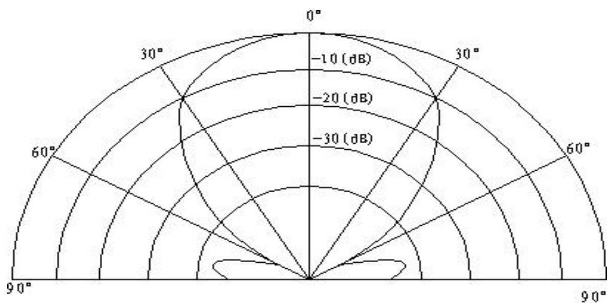
Directivity in Overall Sensitivity
