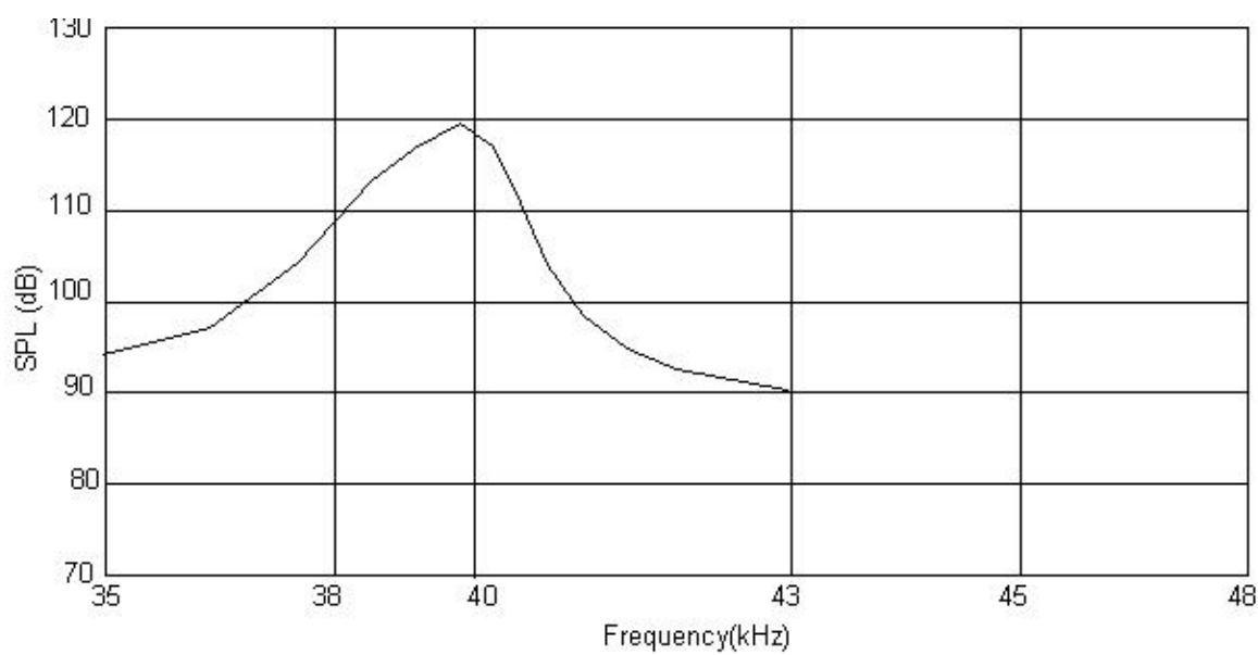
SPL-Frequency Characteristics
