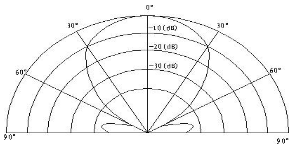
Directivity in Overall Sensitivity
