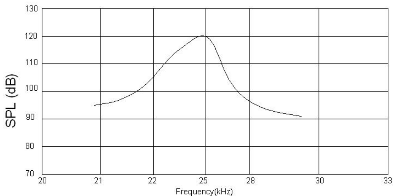
Frequency Characteristics
