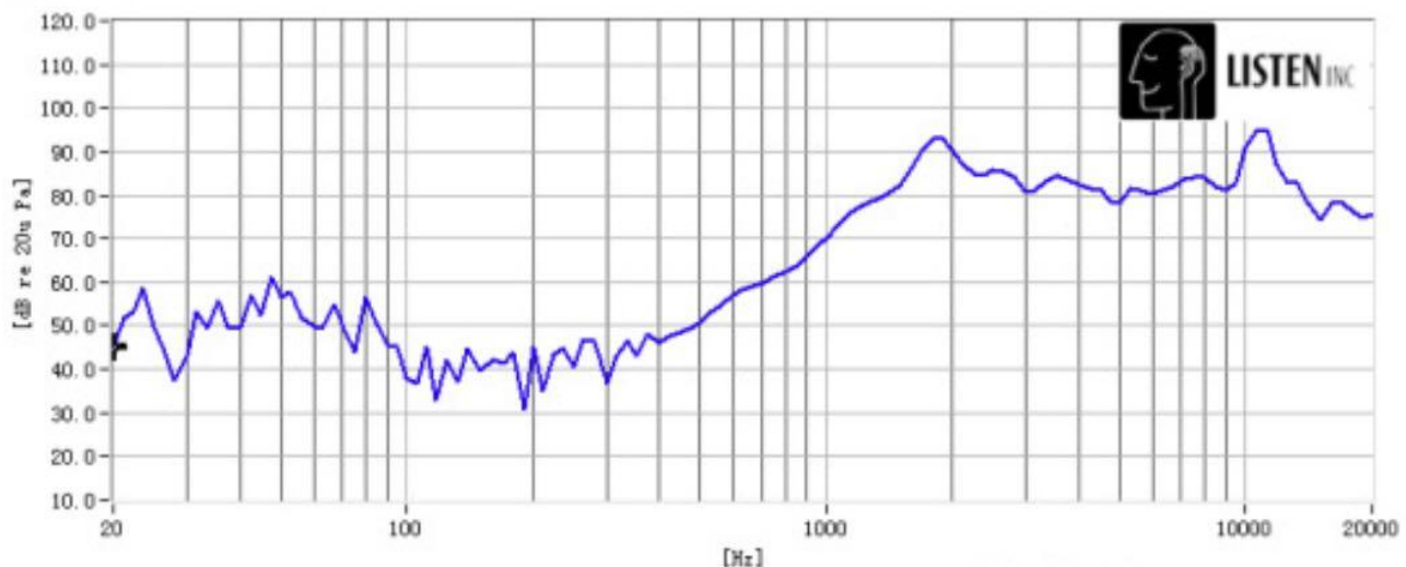
FIG..2(Loud speaker Typical Frequency Response)
