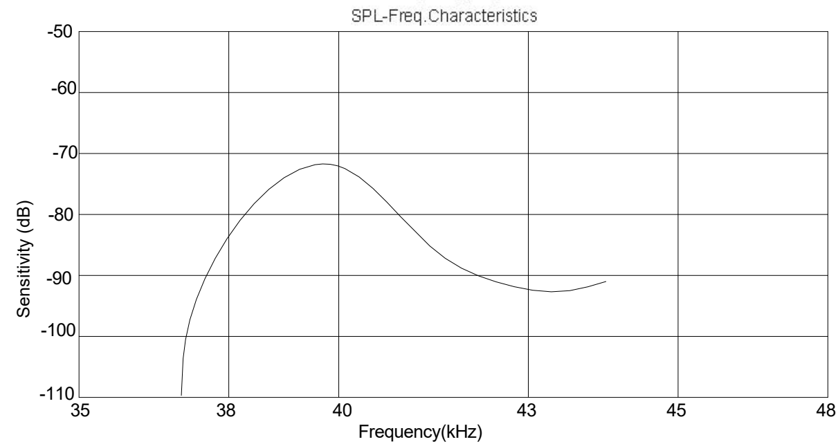
SPL-Frequency Characteristics
