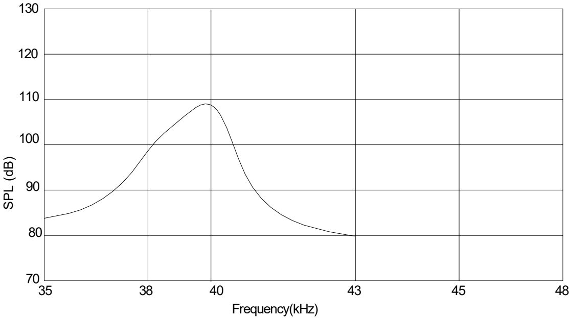
SPL-Frequency Characteristics
