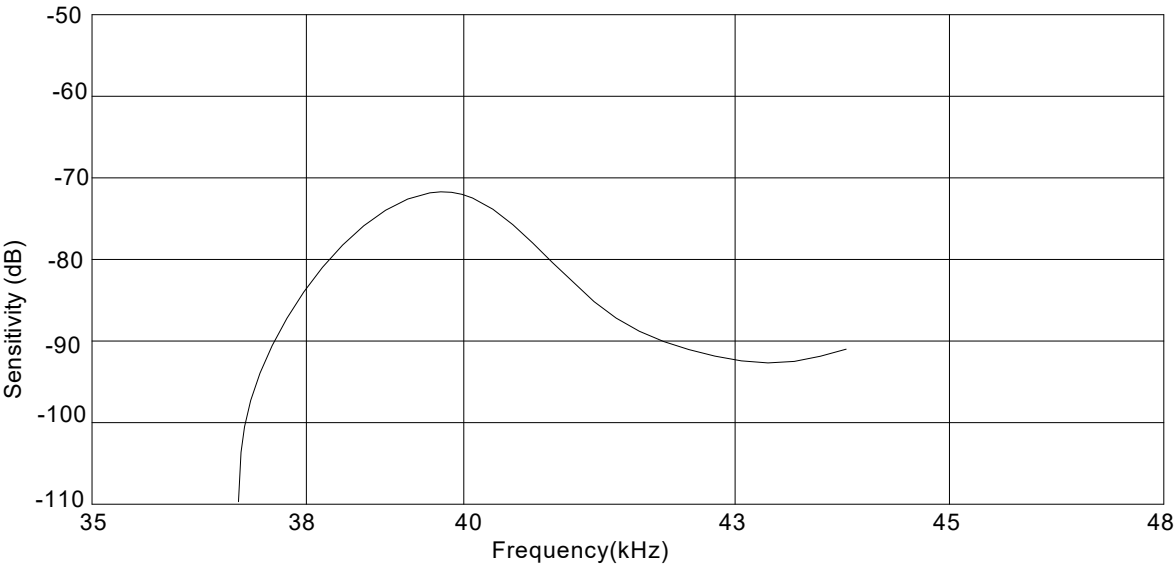
SPL-Frequency Characteristics
