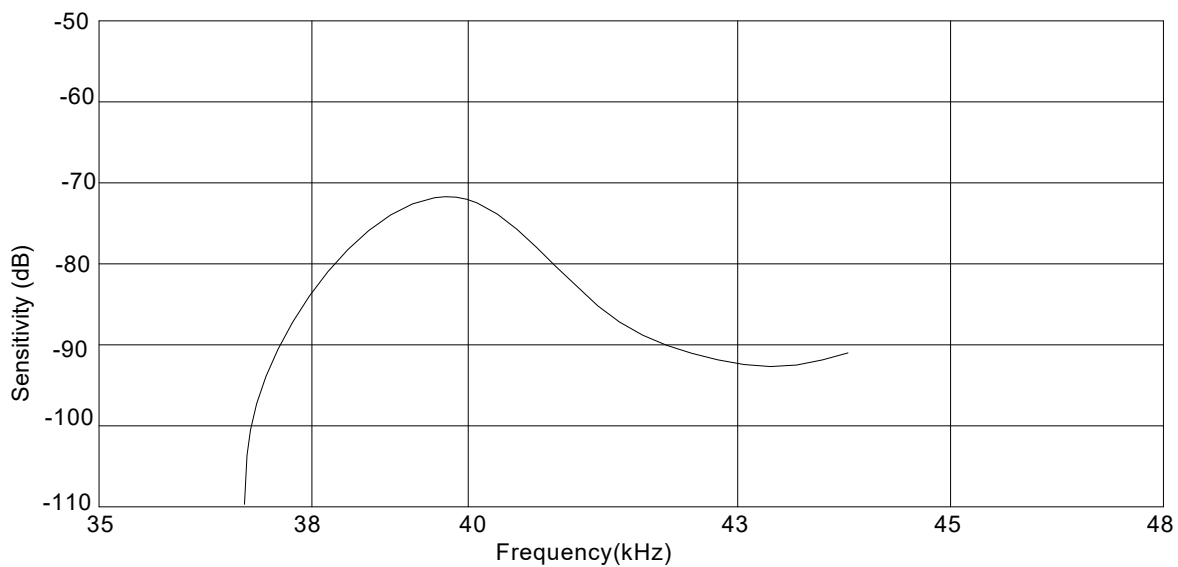
SPL-Frequency Characteristics
