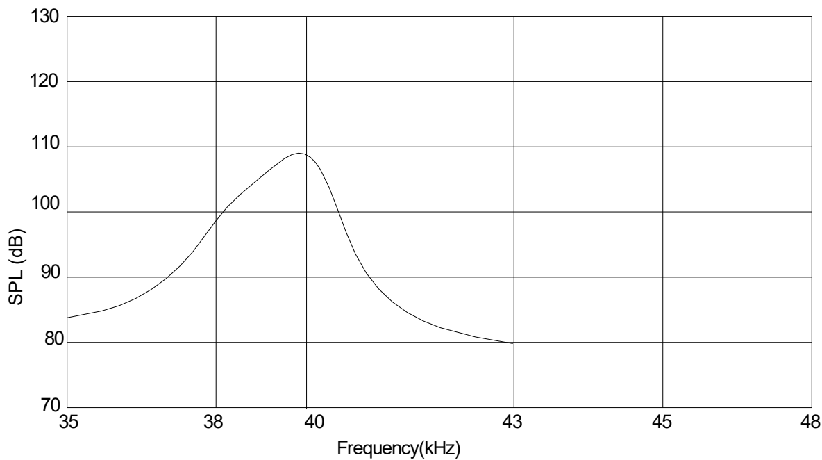
SPL-Frequency Characteristics
